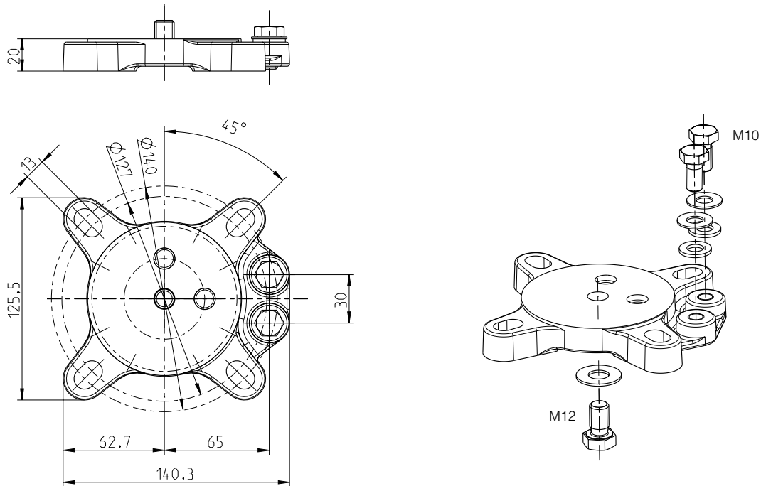
Type 2149 4-points reinforced base (aluminium alloy)
