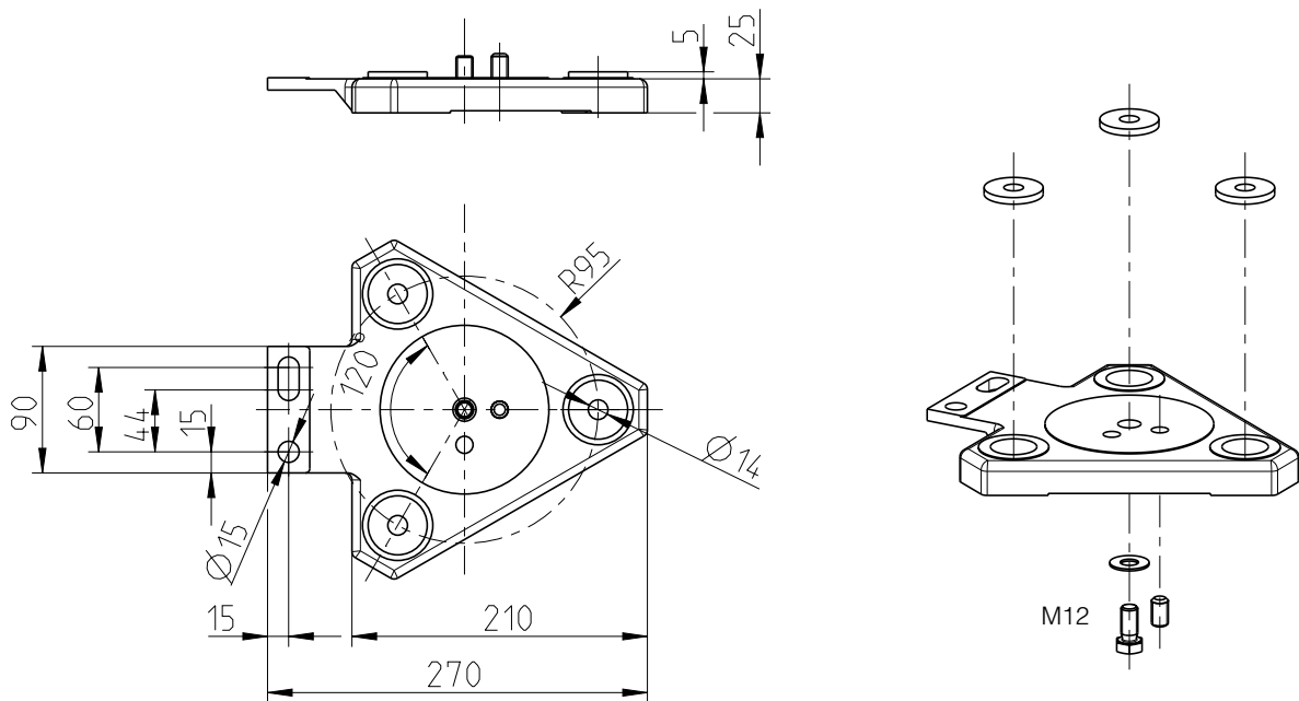
Type 2216 3-points reinforced base R = 95 – (aluminium alloy)
