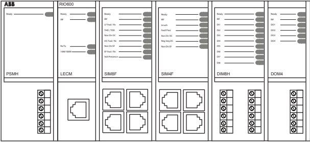
Figure 6. RIO600 configuration: 1 x SIM8F + 1 x SIM4F + 1 x DIM8H + 1 x DOM4
