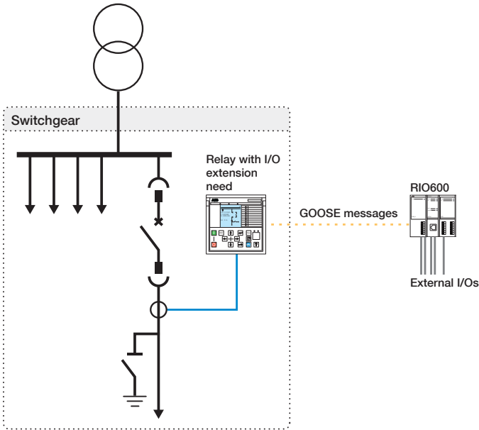
Figure 8. RIO600 as an I/O extension
