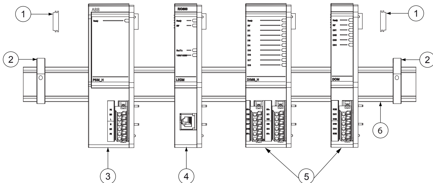
Figure 17. Assembly drawings of RIO600 modules
