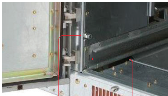
18 Lift truck holding pin Module interlock slot
