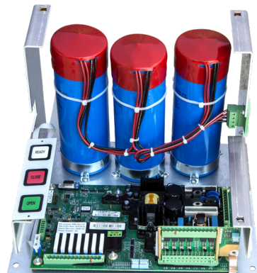
09 R-MAG® circuit breaker control board assembly
