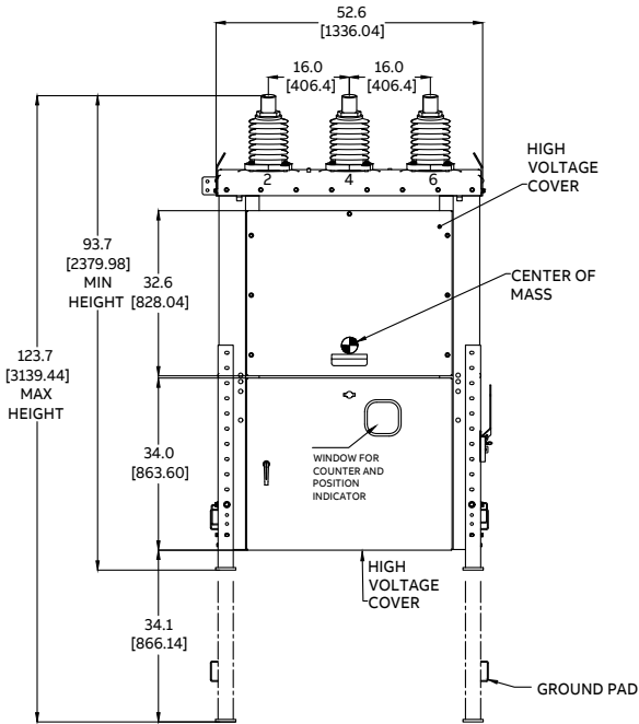
REAR VIEW
