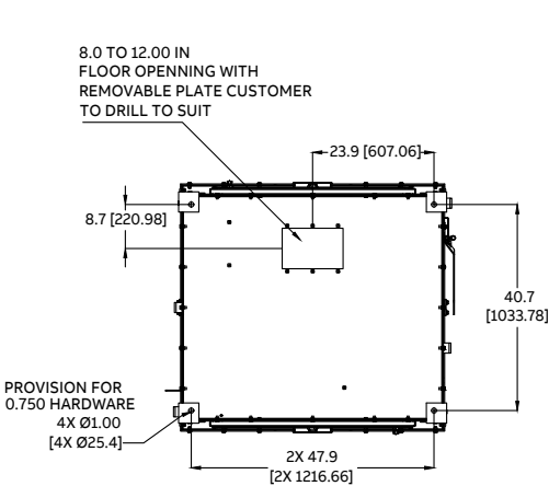
FOUNDATION PLAN
