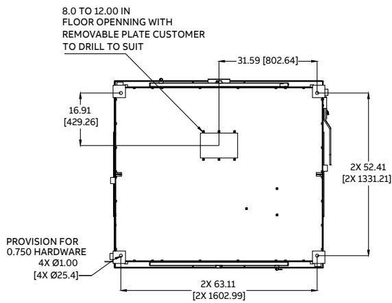
FOUNDATION PLAN
