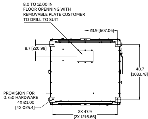
FOUNDATION PLAN
