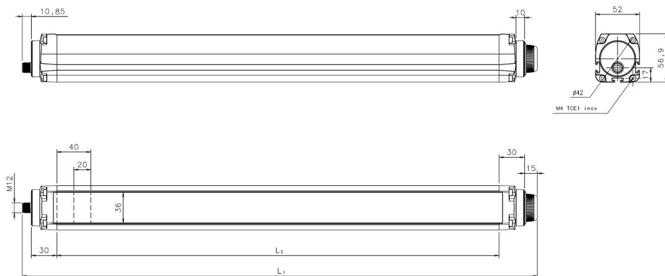
Figure 33 – Active unit
