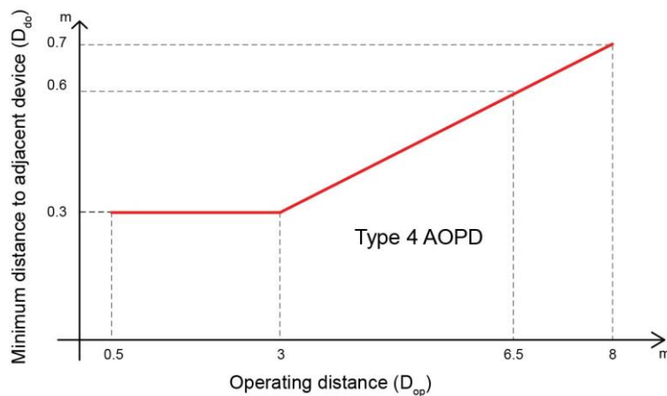
Figure 14 – Minimum distance to an adjacent device as a function of the operating distance
