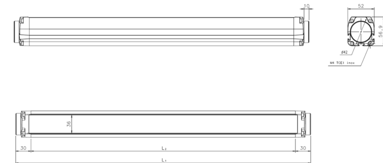
Figure 34 – Passive unit
