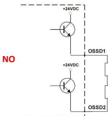
Figure 22 – Incorrect connection of OSSD outputs
