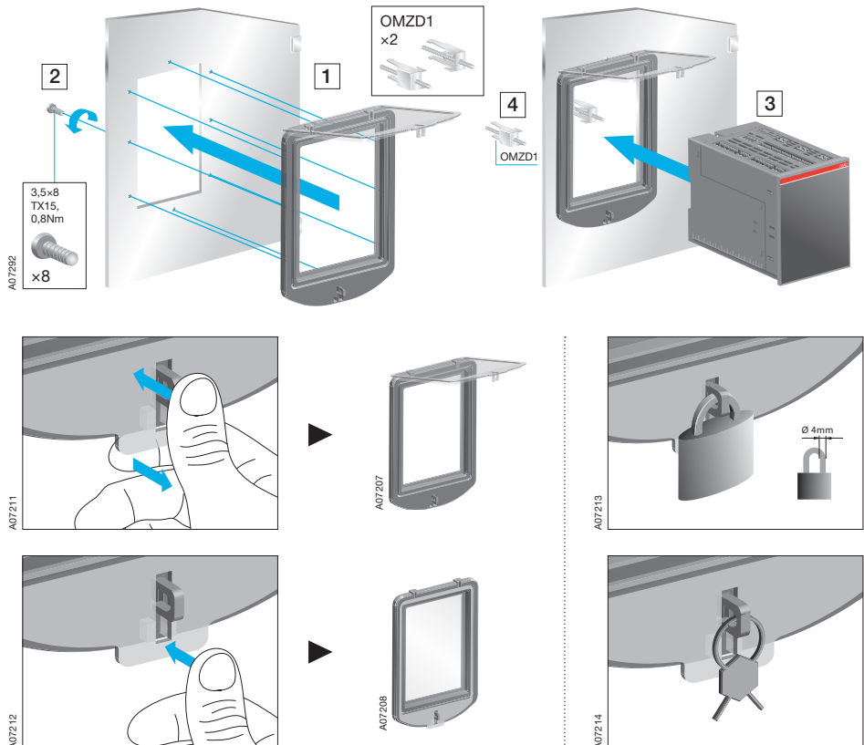
Figure 10.2 Door drilling and mounting of the cover plate OMZC2, when the automatic control unit OMD200 or OMD300 is mounted on the door
