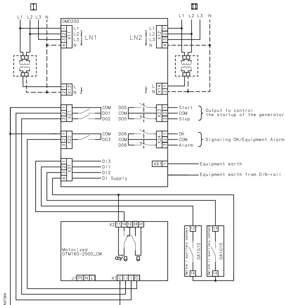
Figure 5.2 Control circuit diagram OMD200 with motorized OTM160...2500_CM_
