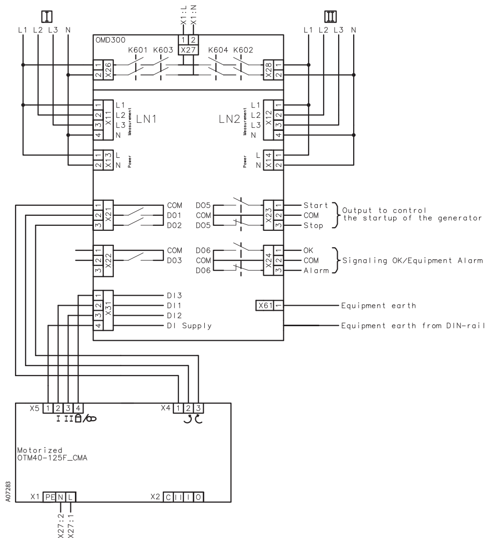
Figure 5.4 Control circuit diagram OMD300 with motorized OTM40...125_CMA_
