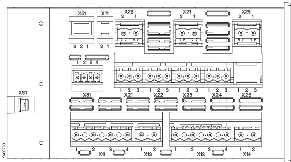
Figure 5.6 Connectors, OMD300
