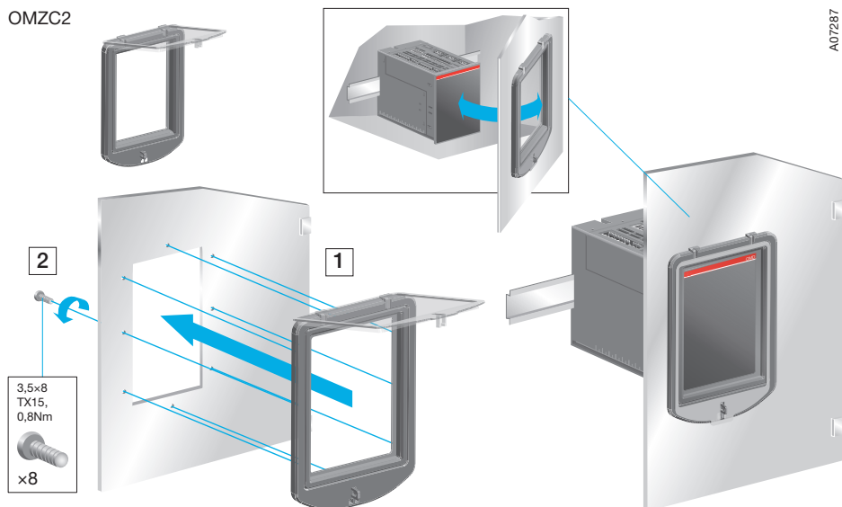
Figure 4.5 Automatic control unit OMD 2 , DIN-rail mounting with the cover plate, door drilling for the cover plate OMZC2, see Accessories, Section 10
