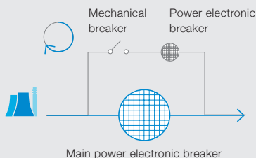
8c Mechanical breaker opens to block upper path
