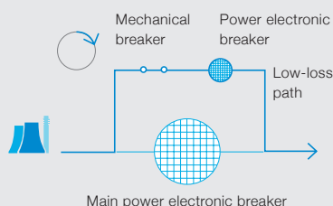
8a Normal operation: Power flow in path with least resistance (results in lower losses)
