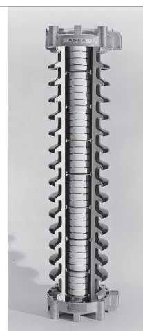
2b ZnO surge arrester (1980s)
