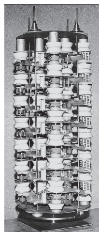
2a XDL 280 A surge arrester (1970s)
