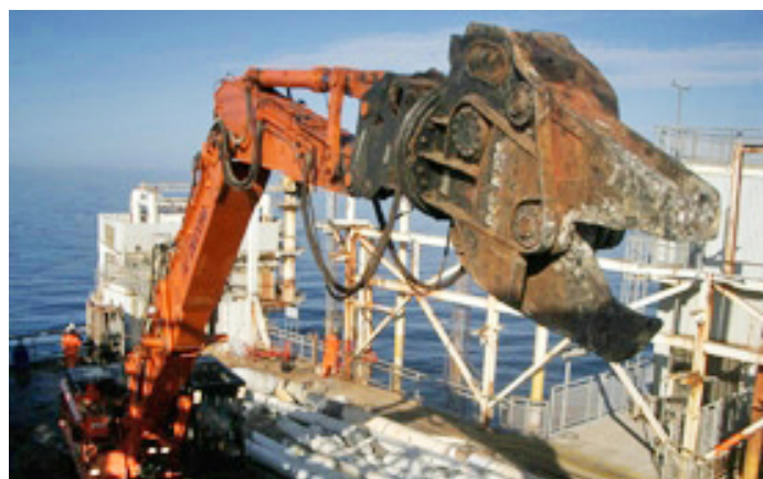
Figure 1: Mobile Shear
