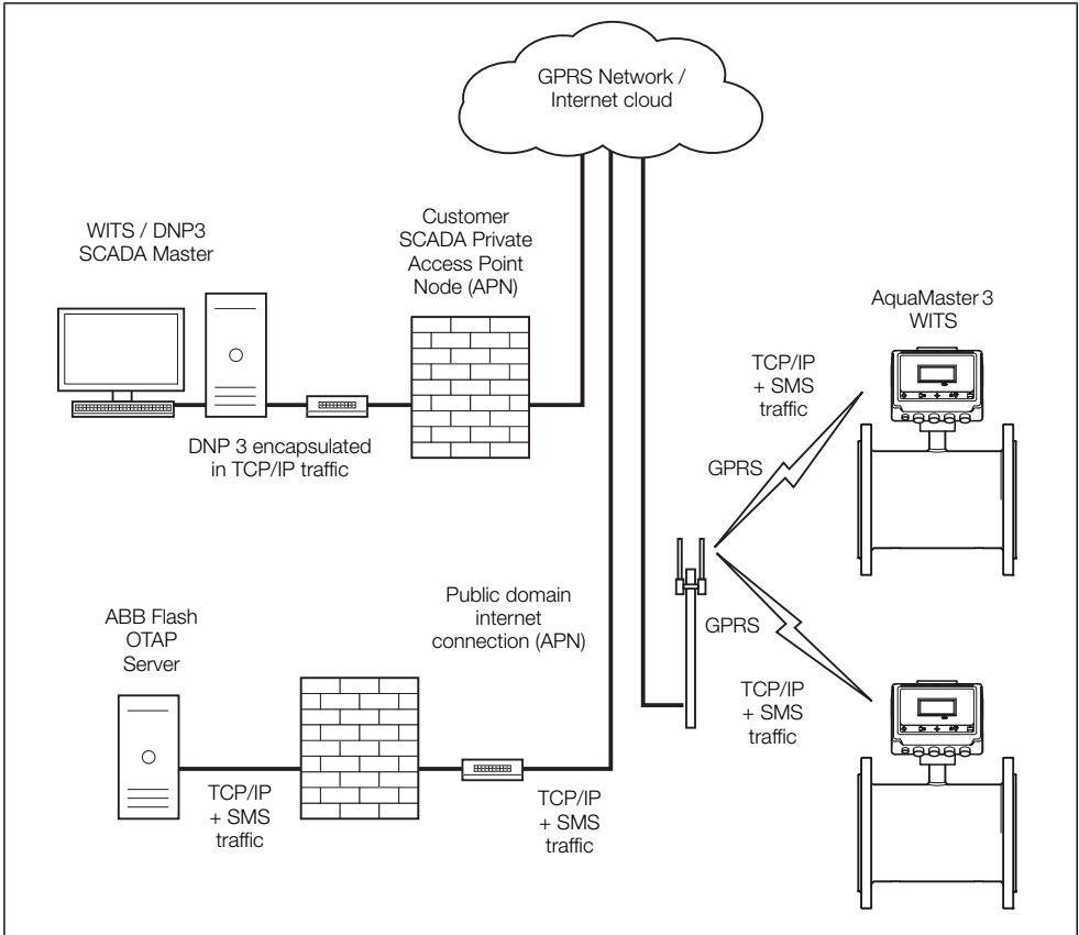
Fig. 7.1 WITS System Architecture
