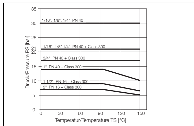
Fig. 6: Liquids
