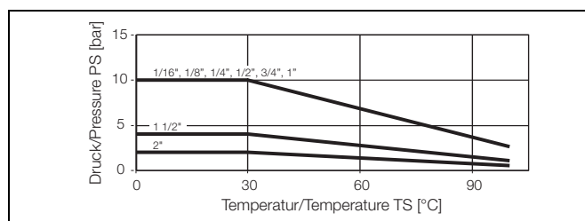
Fig. 3: Gas
