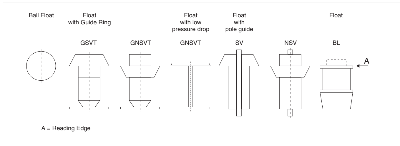
Fig. 7: Float Types
