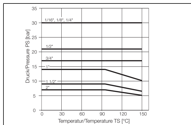
Fig. 2: Liquid
