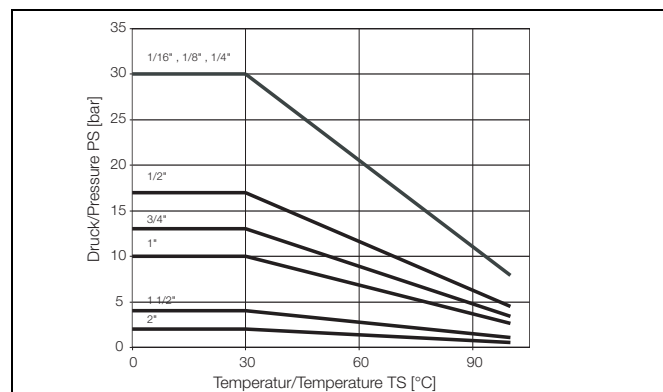
Fig. 1: Gas
