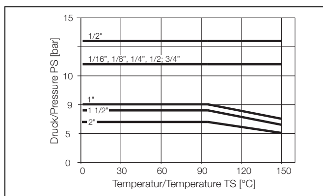
Fig. 4: Liquid
