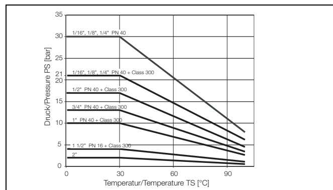
Fig. 5: Gas
