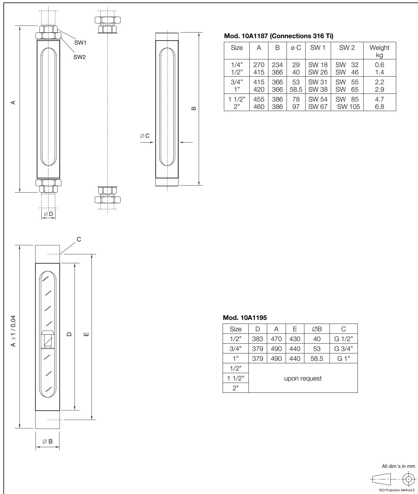
Fig. 12: Dimensions
