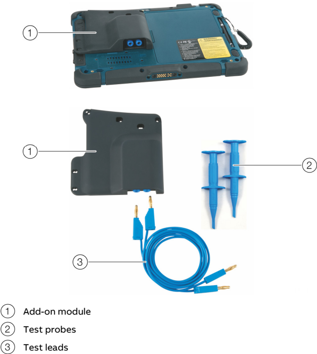
Figure 1: HART® add-on module
