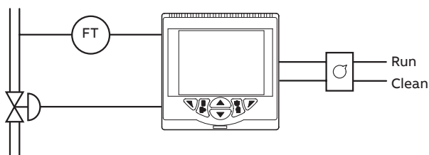
Figure 11 Remote auto / manual switching
