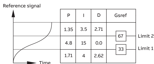
Figure 7 Gain scheduling example
