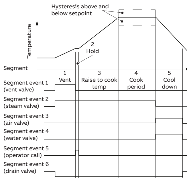
Figure 18 Profile control
