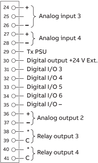
Option board 1
