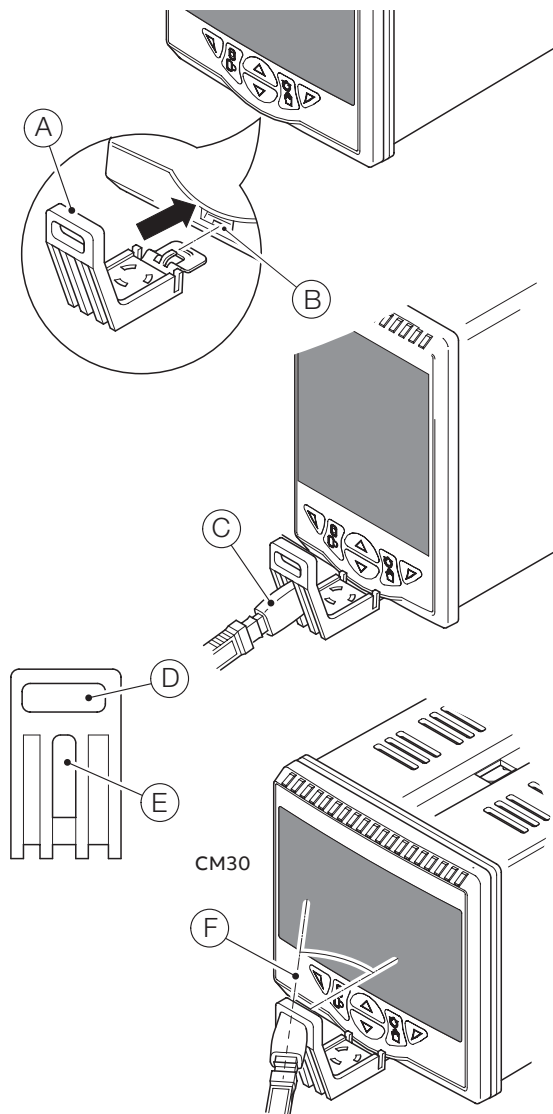
Figure 2 Fitting the IrDA mounting bracket
