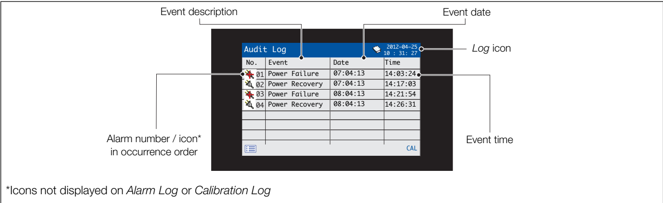
Fig. 6.11 Log page (example of Audit Log shown)
