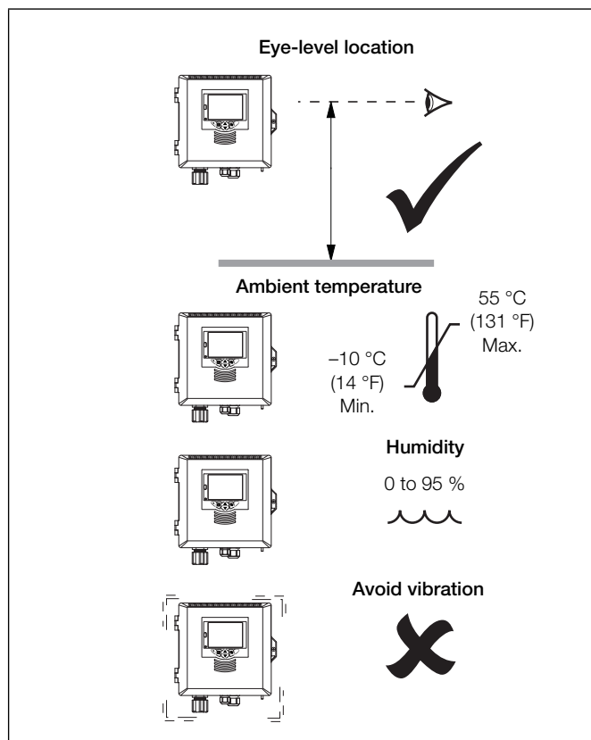
Fig. 3.6 Transmitter location
