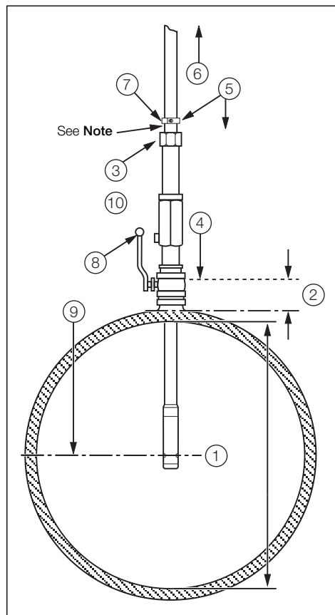
Fig. 3.10 Setting the Insertion Depth – Centre Line Method for Pipe Diameters >1\text{ m} \leq 2\text{ m} ( >40\text{ in.} \leq 80\text{ in.} )
