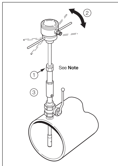
Fig. 3.12 Flow Sensor Alignment
