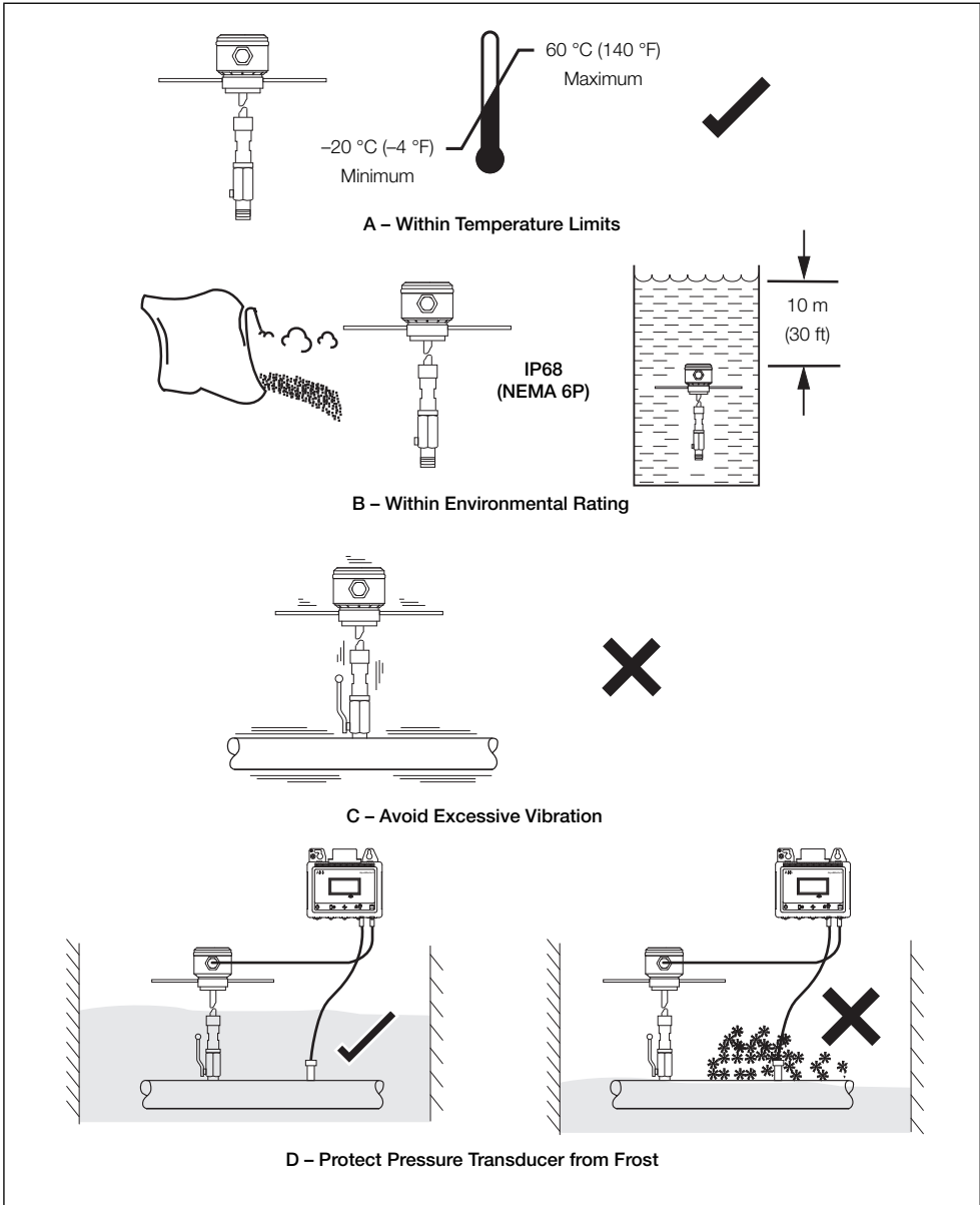
Fig. 3.1 Environmental Requirements
