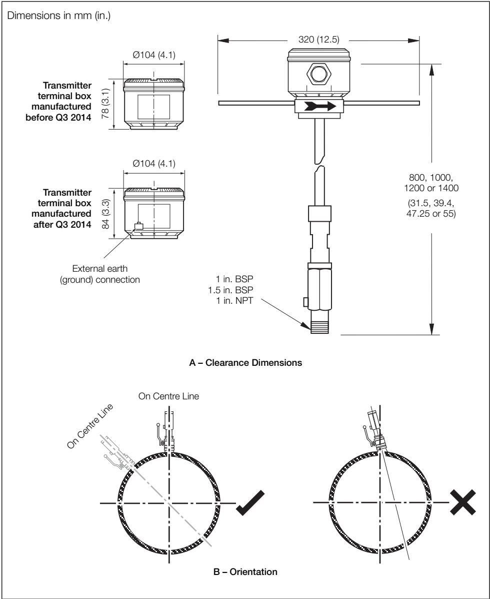
Fig. 3.5 Mechanical Requirements
