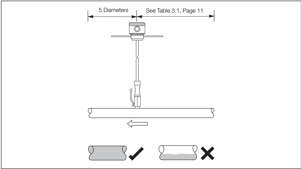
Fig. 3.2 Flow Conditions
