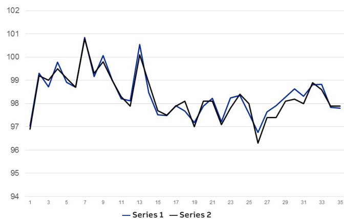
Example validation plot of on-line FT-NIR RON data (Series 1) vs lab test samples (Series 2)
