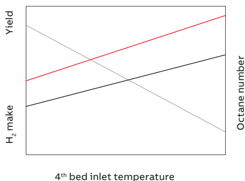
Example operating parameter trade-offs in CCR operation
