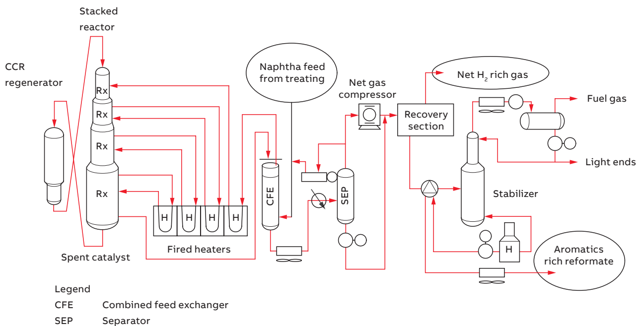
Typical UOP CCR platforming process unit
