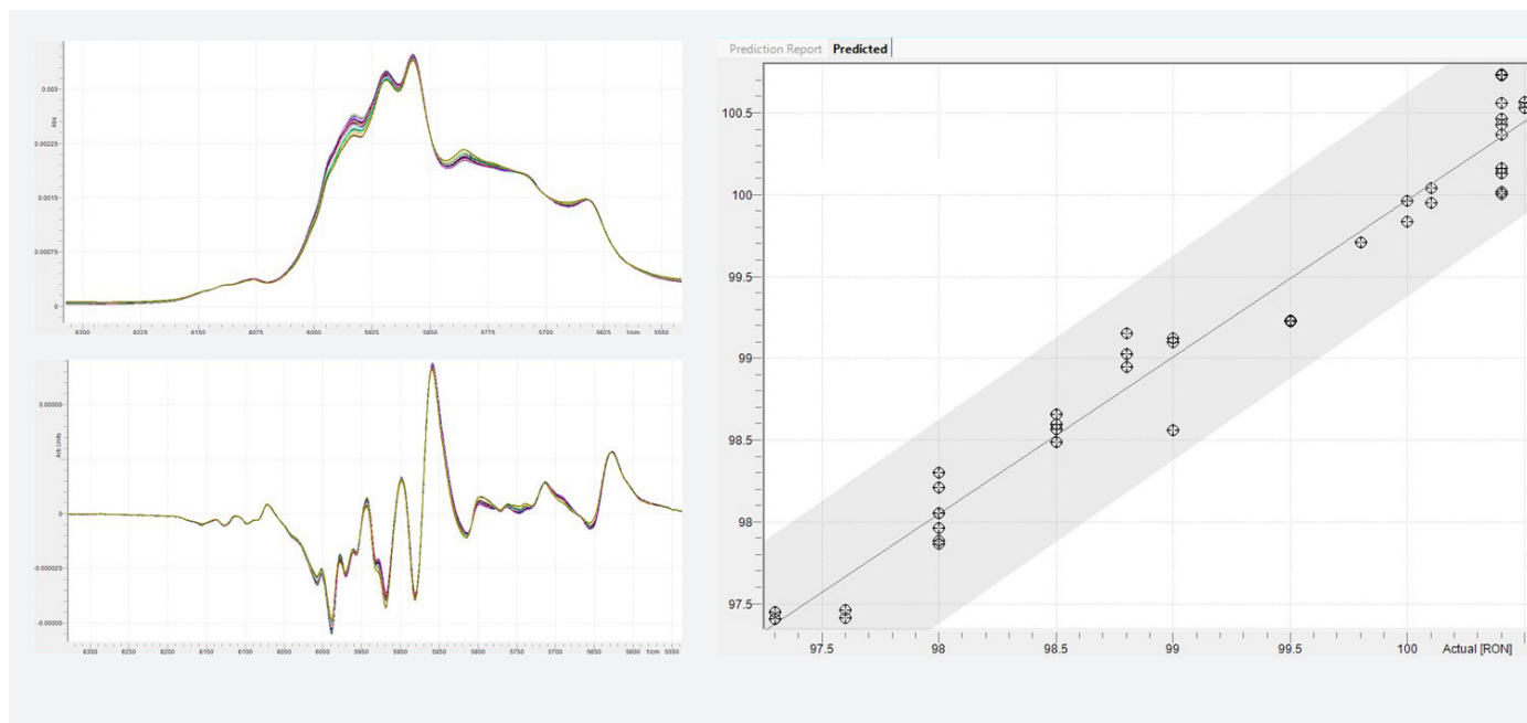
Calibration dataset, 1 st derivative and PLS regression plot for RON
