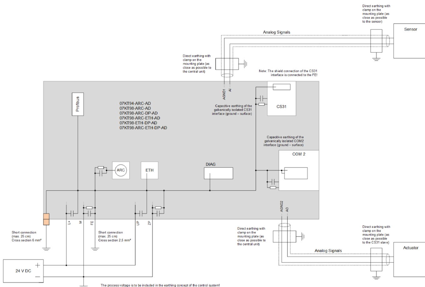
Fig. 3: CPU earthing
