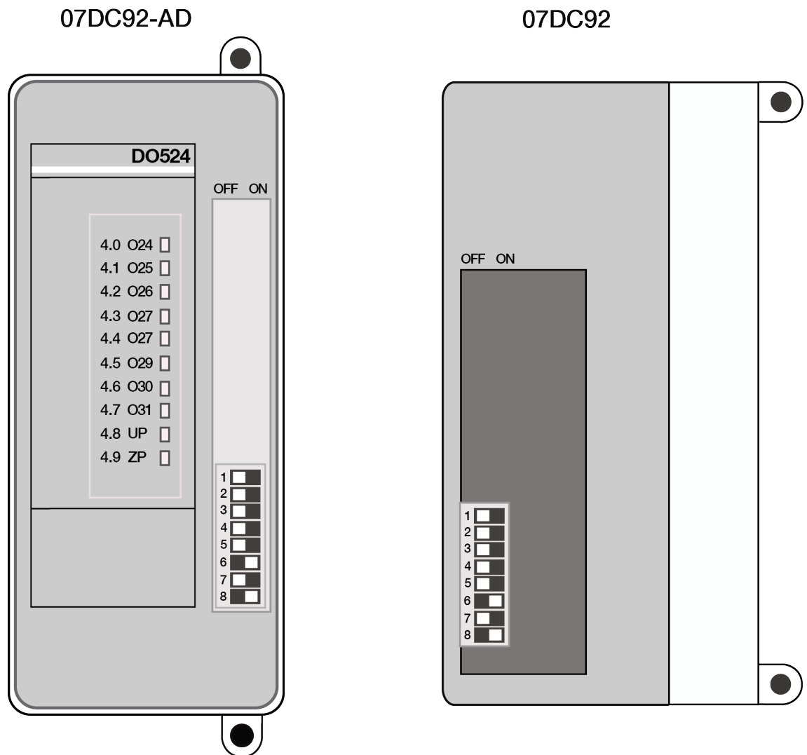
Fig. 50: DIP switch for 07DC92-AD:
