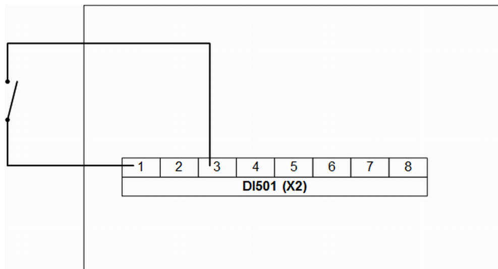
Fig. 90: Connection example: digital input (X2)
