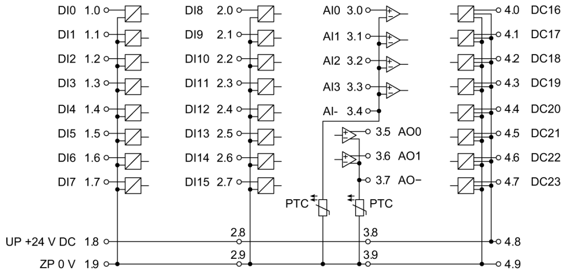
Fig. 22: Circuit arrangement of DA501 module
