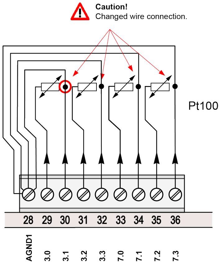
Fig. 31: Connection of Pt100 temperature sensors in 3-wire configuration
