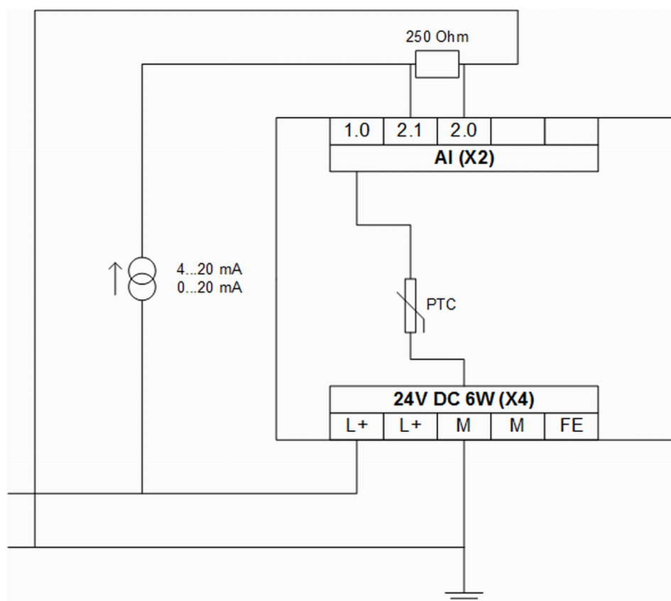
Fig. 60: Current input with external resistor
