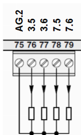
Fig. 34: Connection of output loads (voltage and current) to analog outputs
