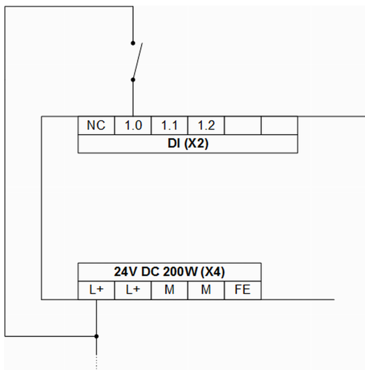
Fig. 40: Connection example: digital input
