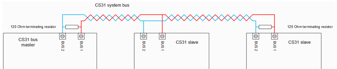
Fig. 4: Bus topology with CS31 bus master on the side
