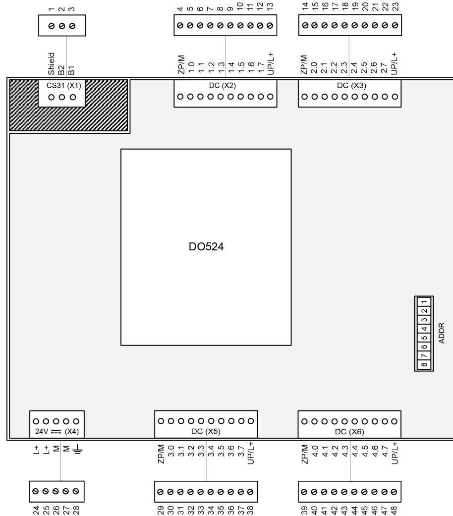
Fig. 48: Electrical connection
