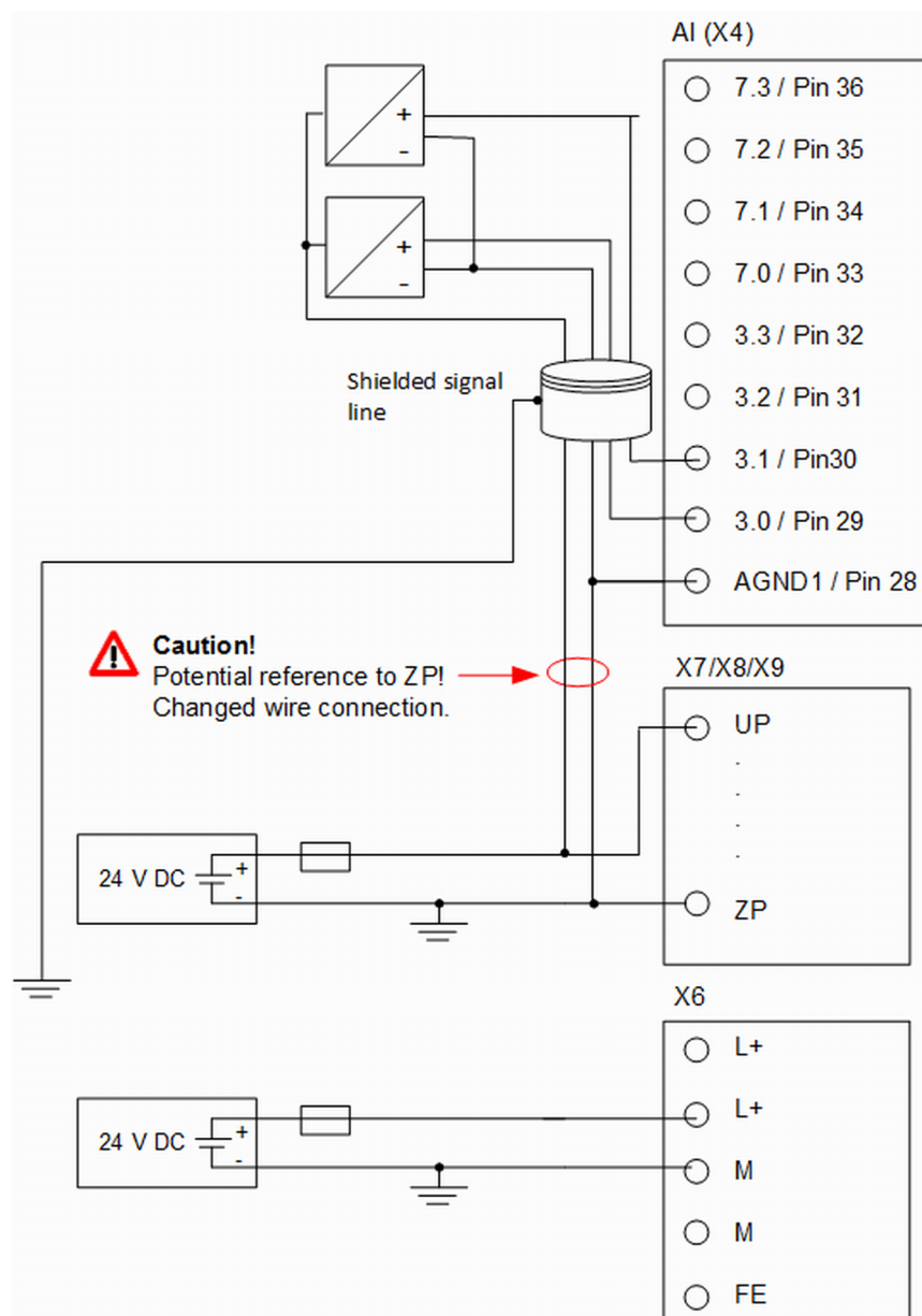
Fig. 28: Voltage input with externally supplied 3-wire voltage sensors
