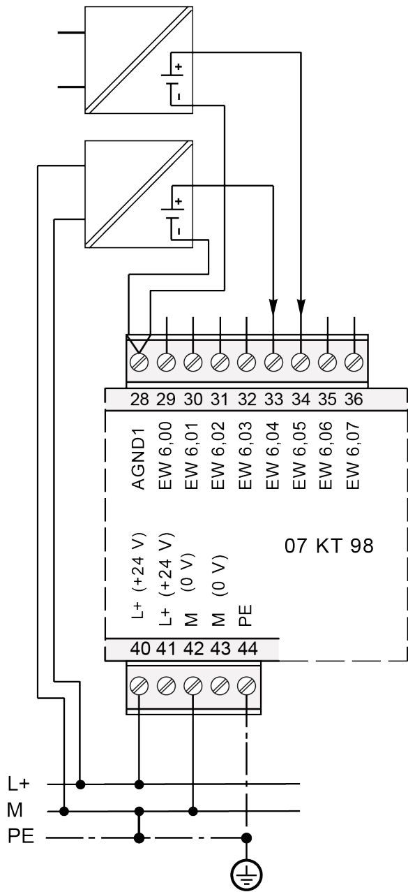
Fig. 27: 07KT98_Measuring_Ranges \pm 10\text{ V} / 0 \dots 10\text{ V}
