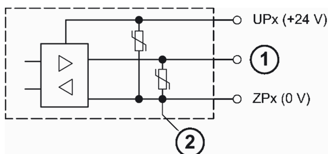
Fig. 25: Circuit arrangement
