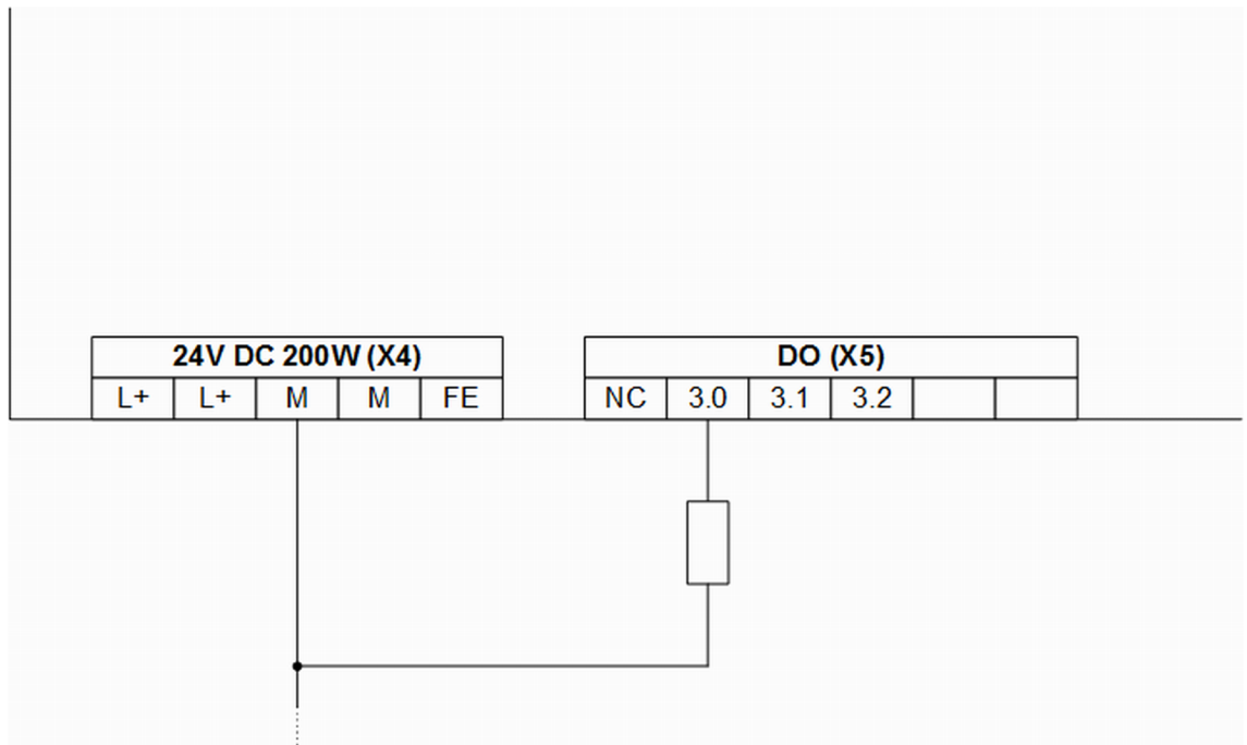
Fig. 41: Connection example: digital output
