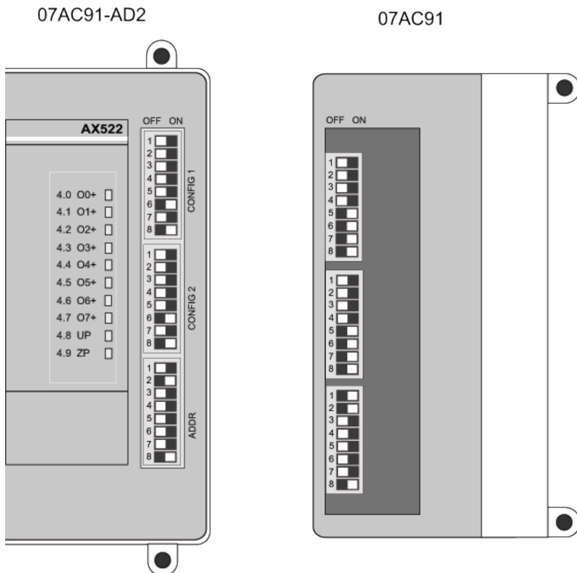
Fig. 82: DIP switch for 07AC91-AD2
