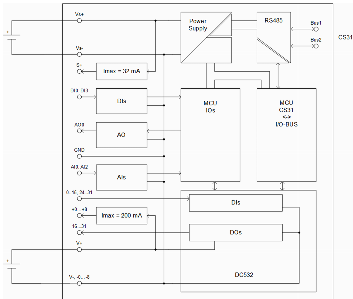
Fig. 94: Schematic diagram
