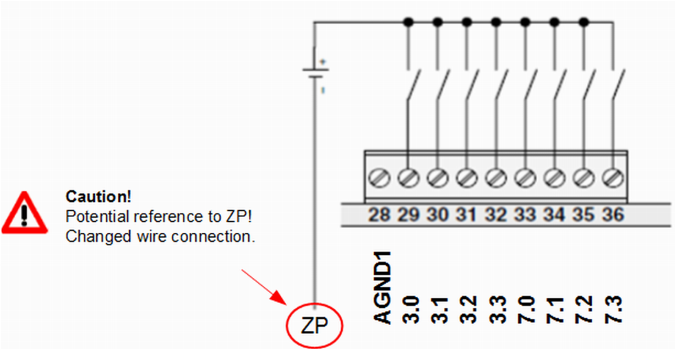
Fig. 32: Use of analog inputs as digital inputs
