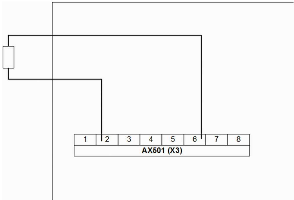
Fig. 92: Connection example: Voltage output
