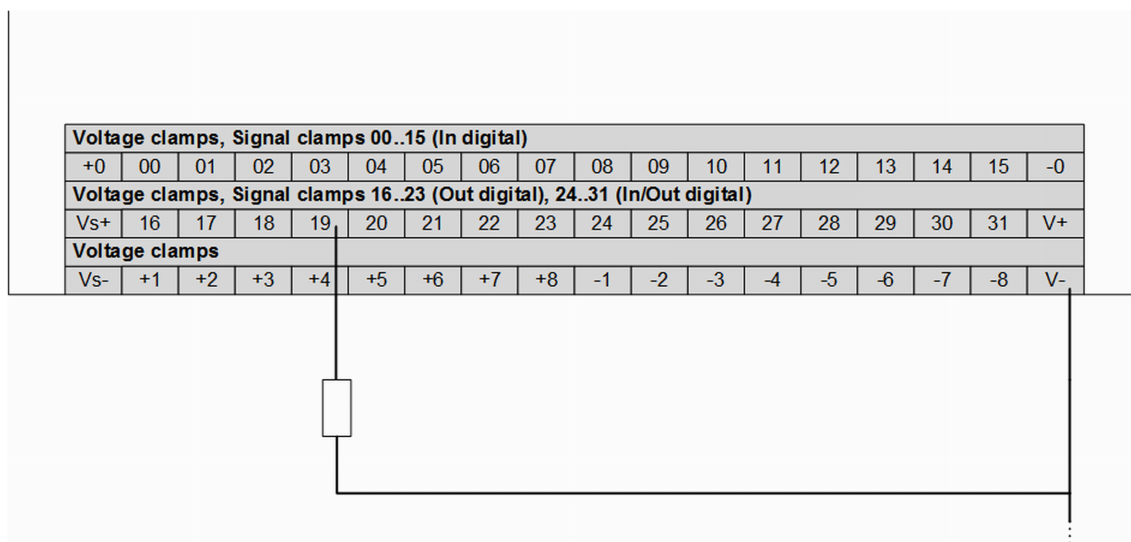
Fig. 89: Connection example: digital output
