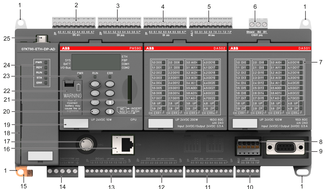
Fig. 17: 3ADR333186F0015_07KT98-ETH-DP-AD_Front
