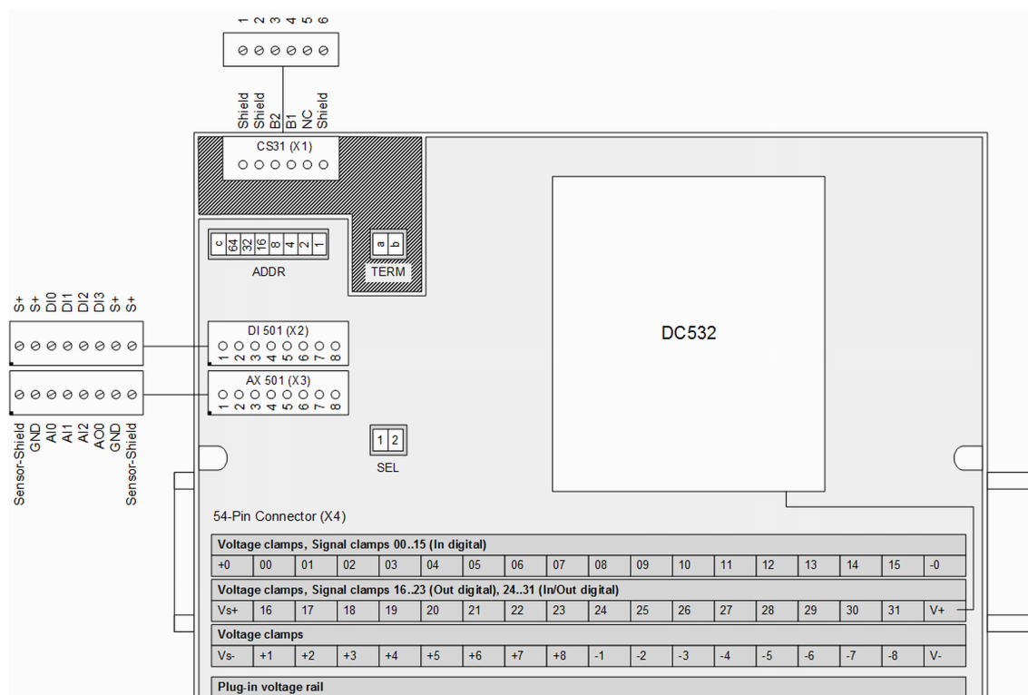
Fig. 87: Electrical connection
