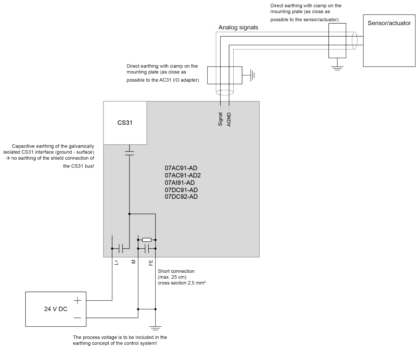
Fig. 1: Earthing of devices 07AC91-AD, 07AC91-AD2, 07AI91-AD, 07DC91-AD and 07DC92-AD
