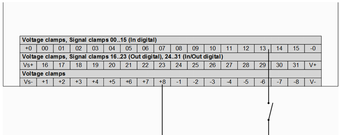
Fig. 88: Connection example: digital input (X4)
