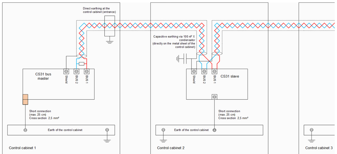
Fig. 7: Direct earthing of CS31 bus master and capacitive CS31 slave
