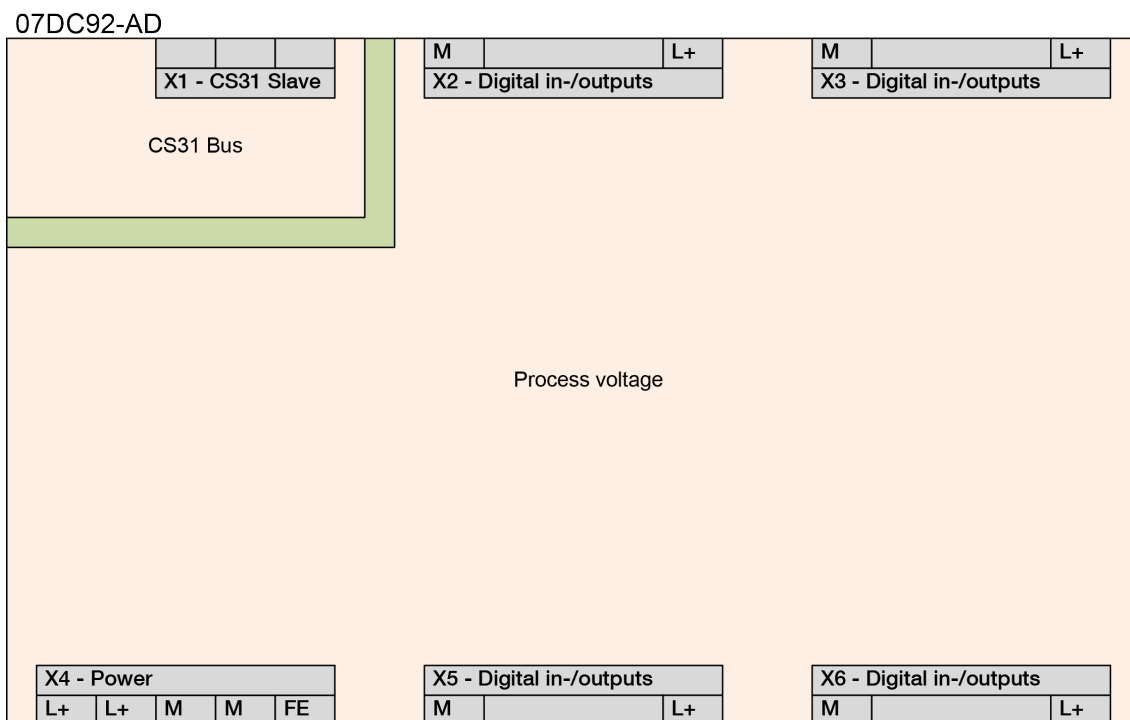
Fig. 53: Process voltage connections - 07DC92-AD
