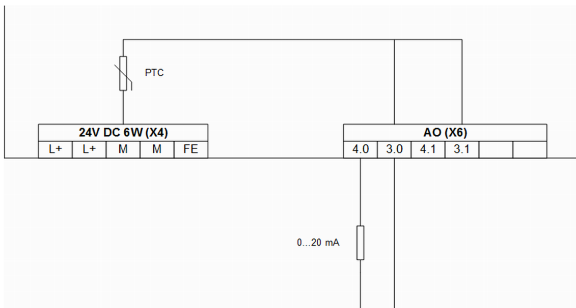
Fig. 81: Current output
