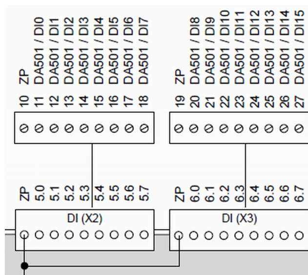
Fig. 20: Arrangement of the 16 digital inputs
