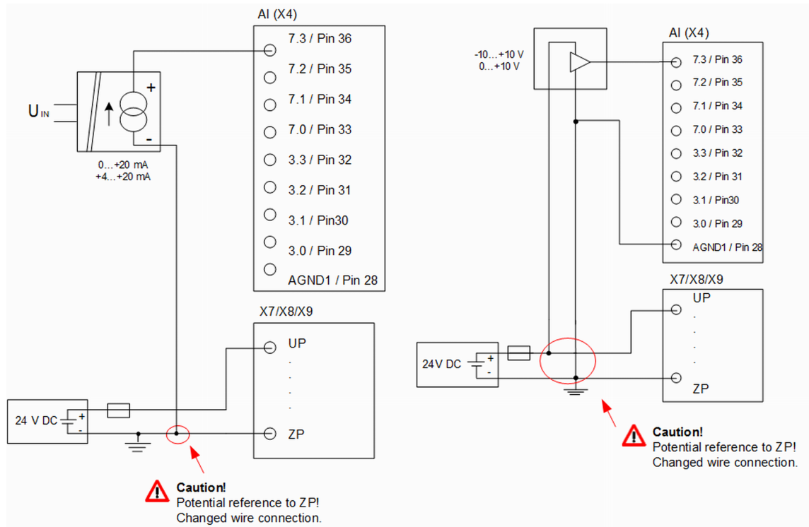
Fig. 30: Connection of current sensors 0 ... 20 mA to the analog inputs
