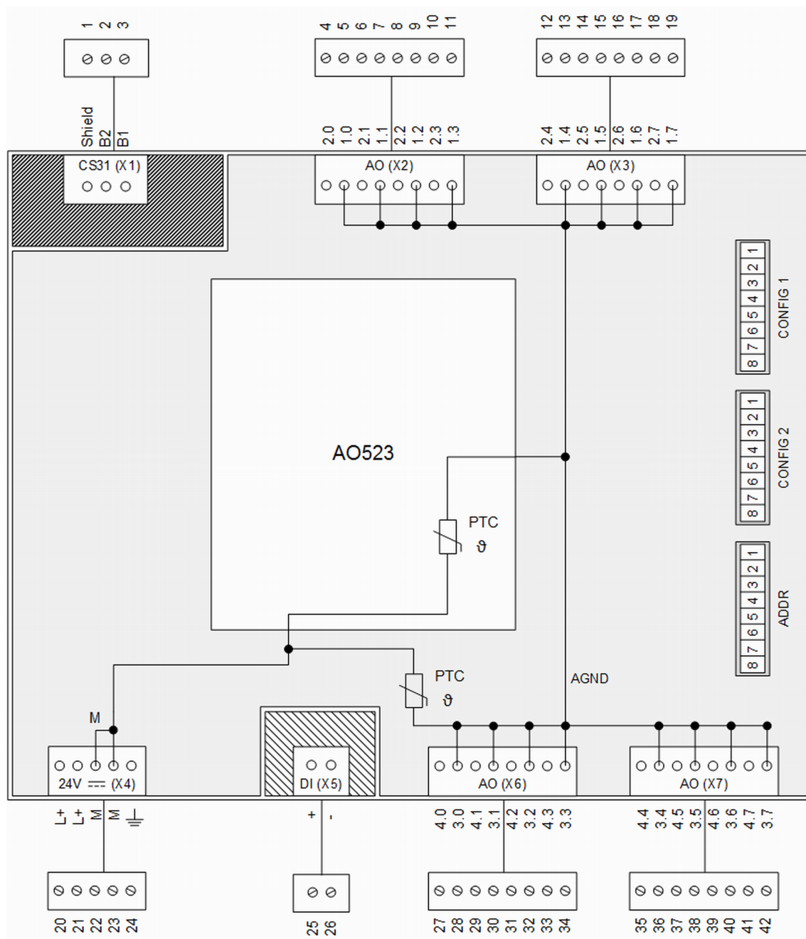
Fig. 69: Electrical connection
