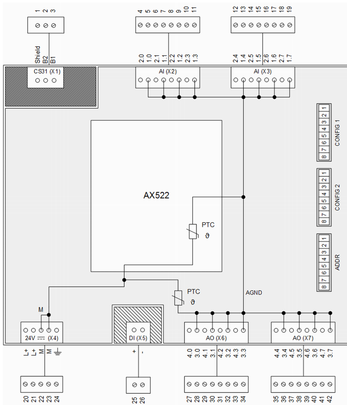
Fig. 77: Electrical connection
