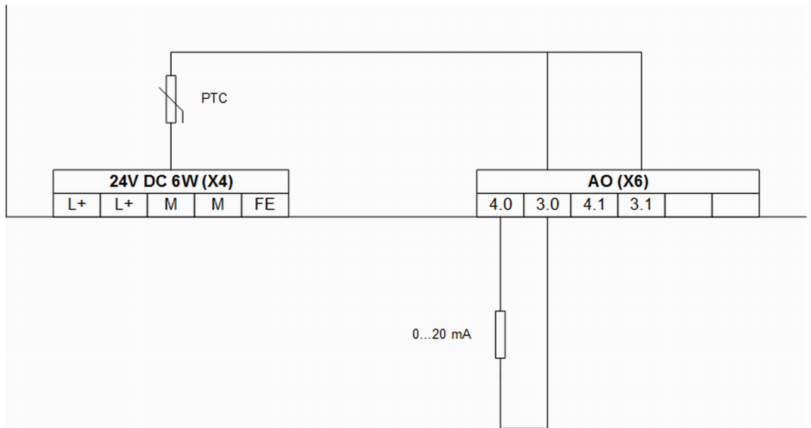
Fig. 71: Current output
