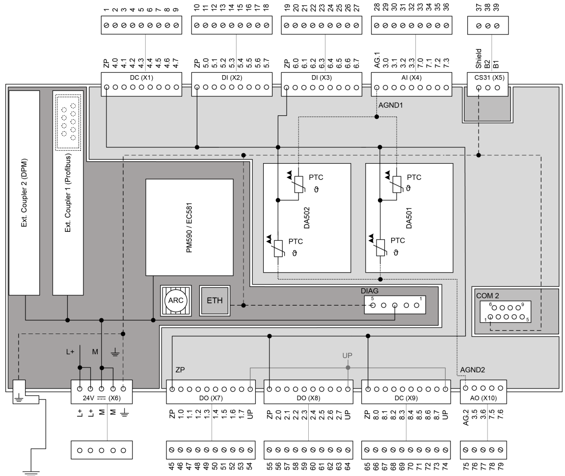
Fig. 18: Terminal assignment 07KT9x-AD
