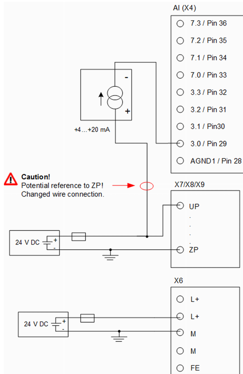
Fig. 29: Connection of current sensors 4 ... 20 mA to the analog inputs
