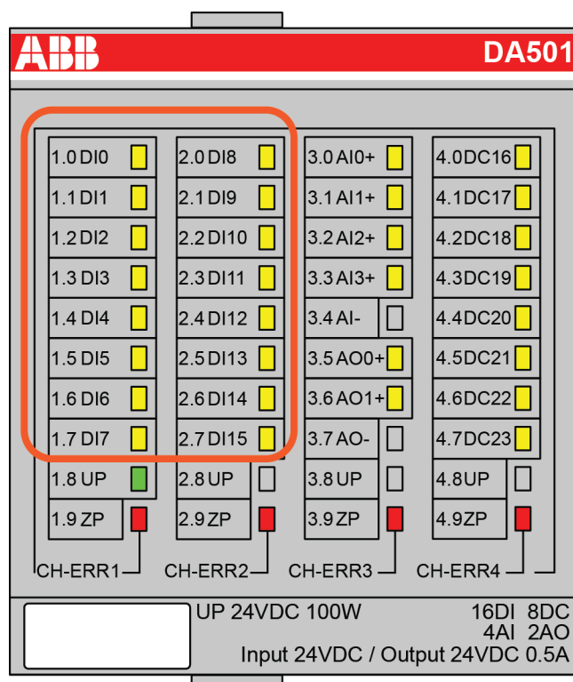
Fig. 21: DA501 LED status indication
