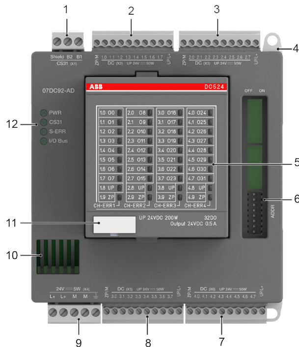
Fig. 46: 3ADR333196F0015_07DC92-AD_Front
