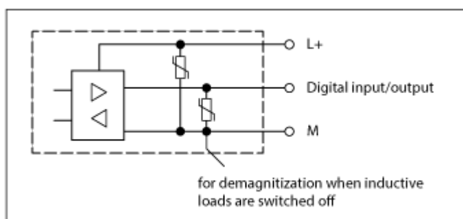
Fig. 54: Protective circuits inputs/outputs
