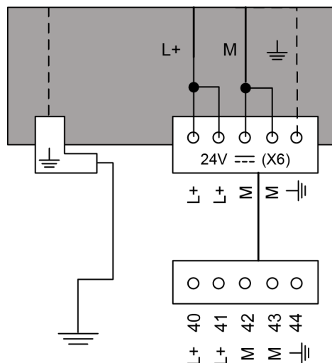
Fig. 19: Connection of the supply voltage
