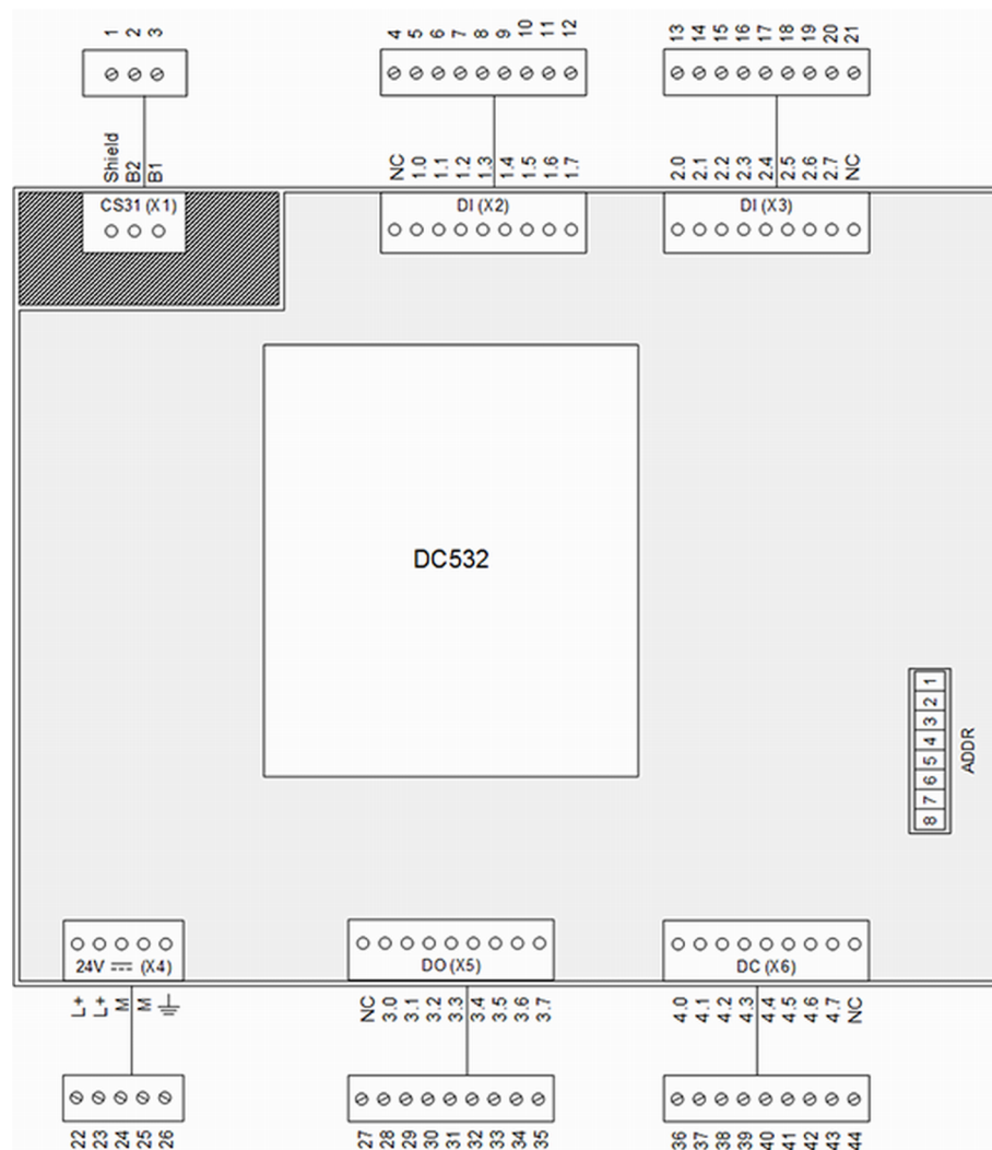
Fig. 39: Electrical connection
