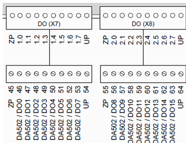
Fig. 23: Arrangement of digital outputs
