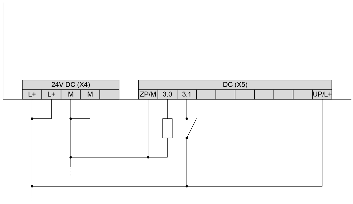
Fig. 49: Connection example: digital output
