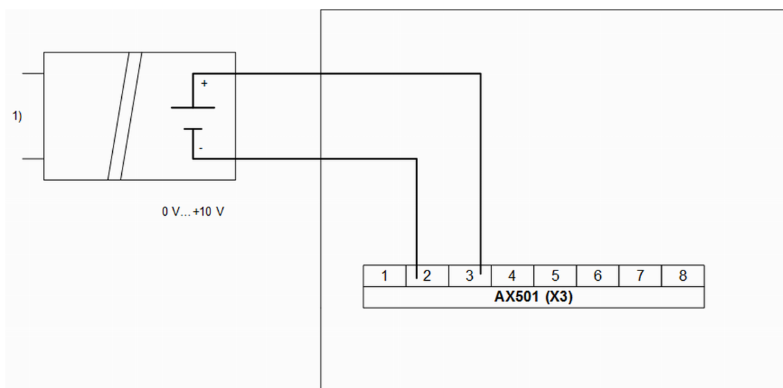
Fig. 91: Connection example: Voltage input
