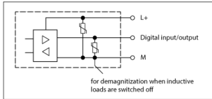
Fig. 44: Protective circuits inputs/outputs
