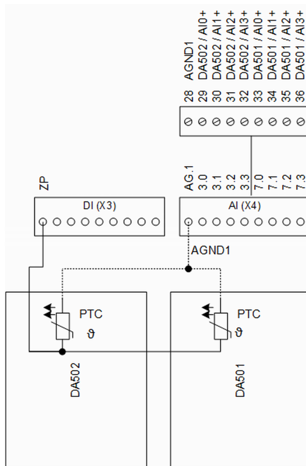
Fig. 26: Arrangement of the analog inputs
