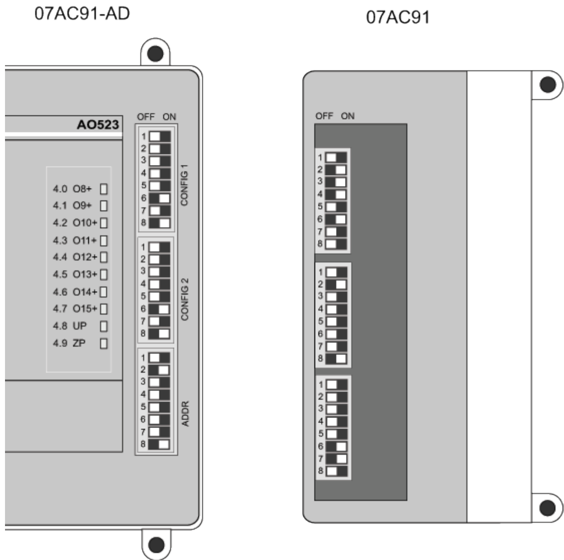
Fig. 72: DIP switch for 07AC91-AD
