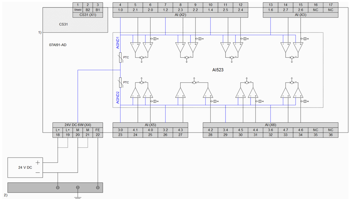
Fig. 58: Electrical connection
