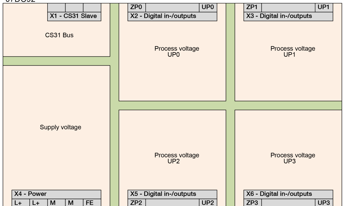
Fig. 52: Process voltage connections - 07DC92
