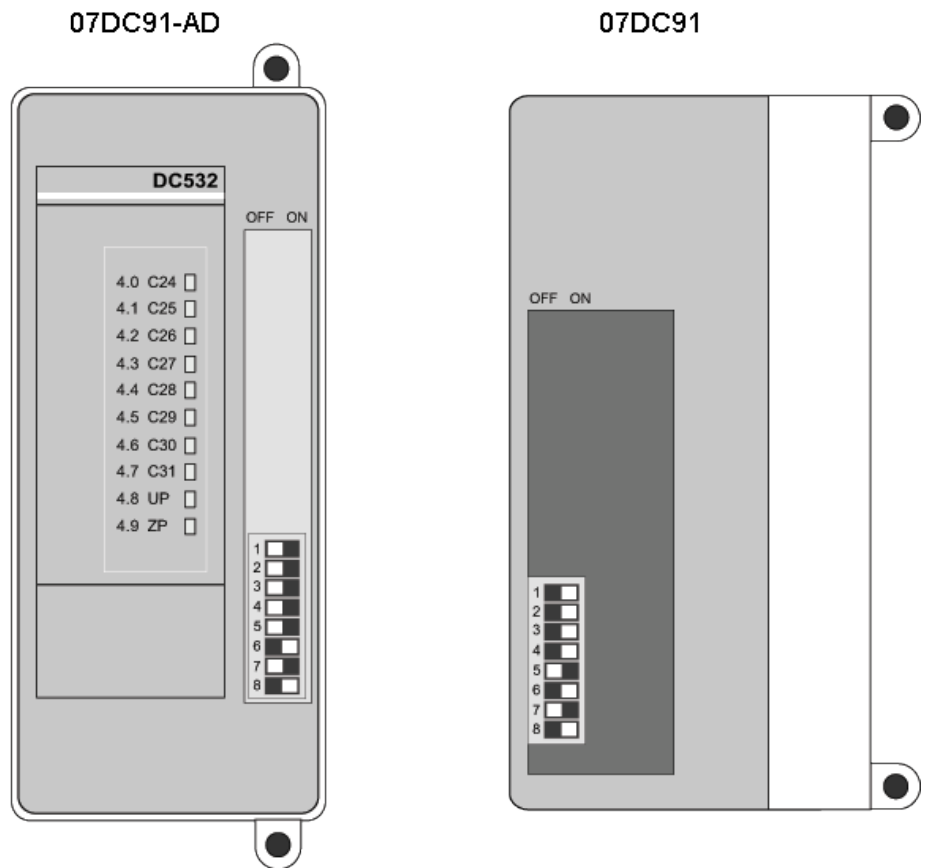
Fig. 42: DIP switch for 07DC91-AD
