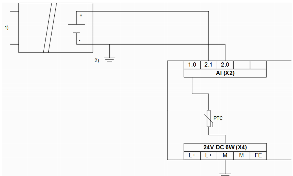
Fig. 59: Differential voltage input
