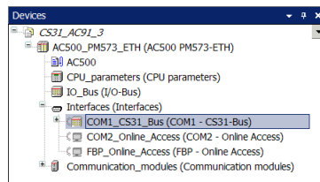
Fig. 11: CS31 bus master
