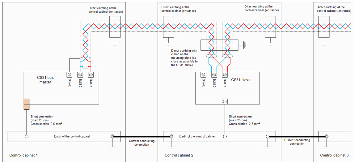
Fig. 6: Direct earthing of CS31 bus master and CS31 slave
