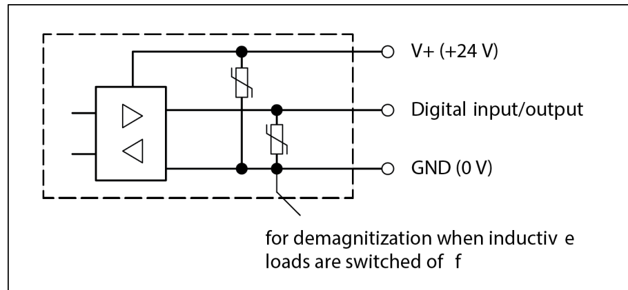
Fig. 98: Protective circuits inputs/outputs
