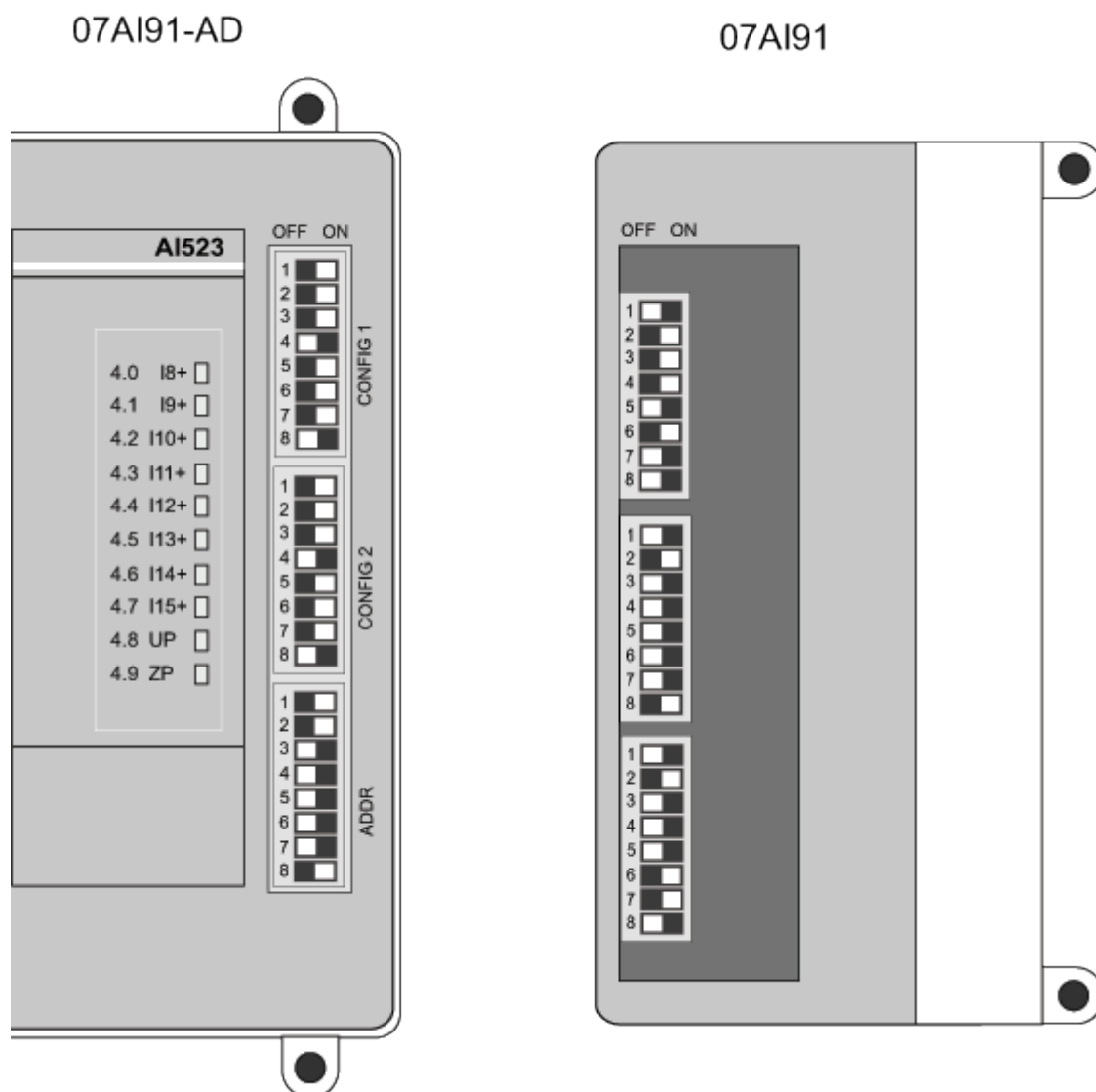
Fig. 62: DIP switch for 07AI91-AD
