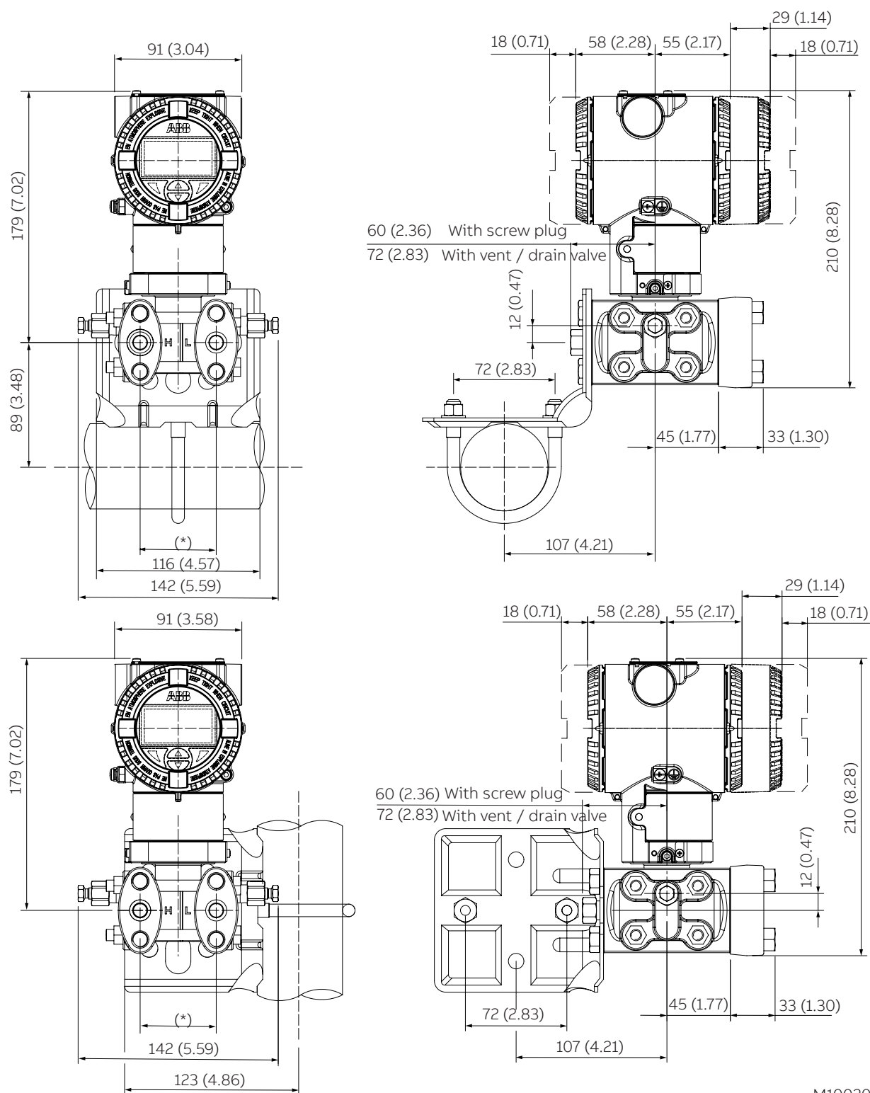
Figure 3: Transmitter with mounting bracket, for vertical or horizontal mounting on 60 mm (2 in) pipe
