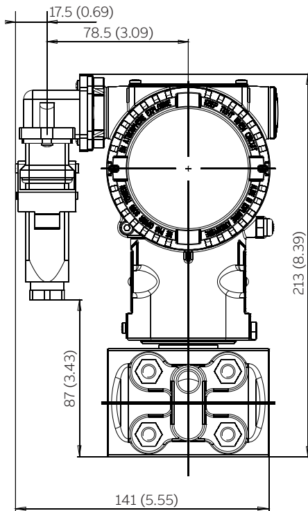
Figure 9: Harting Han connection – HART version
