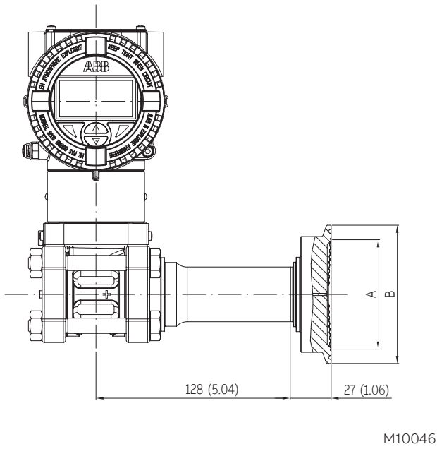
Figure 22 266MRT with barrel housing and direct mount seal S26SS Triclamp (For dimensions of S26 seals refer to the S26 datasheet)
