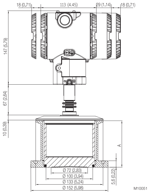
Figure 29 266GRT/ART with barrel housing and direct mount seal S26SS Sanitary extended
