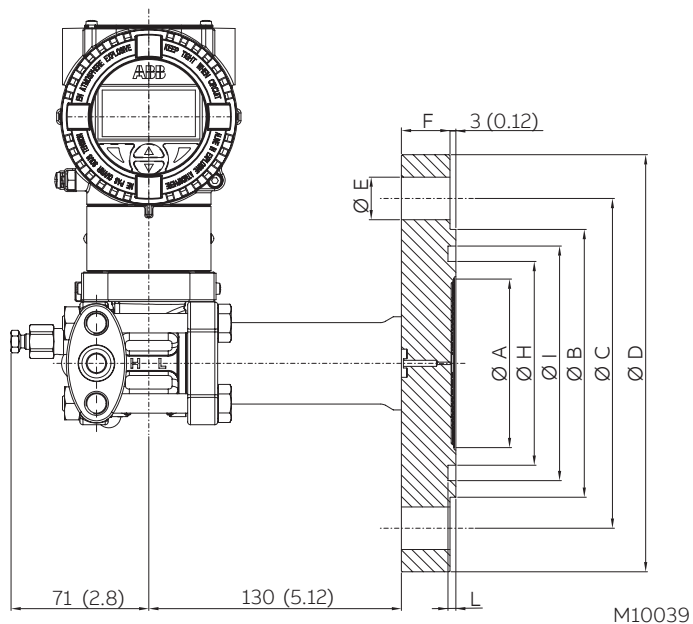
Figure 13 266MRT with barrel housing and direct mount seal S26FA/S26FE fixed flange Raised Face flush diaphragm EN 1092/1 Form D (For dimensions of S26 seals refer to the S26 datasheet)
