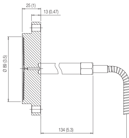
Figure 15: Chemical Tee remote seal
