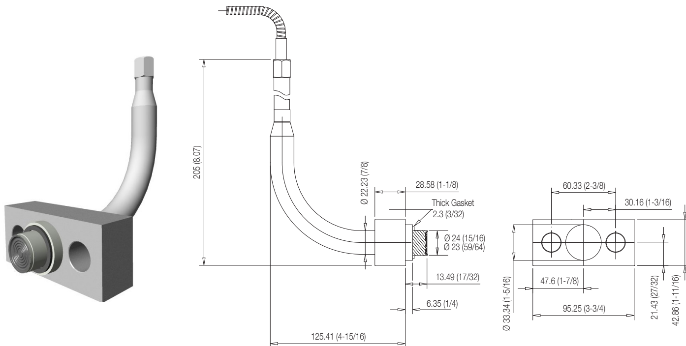
Figure 26: Bracket – type 89
