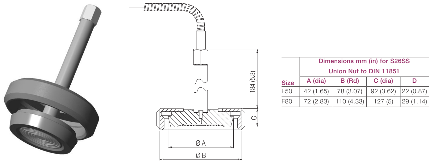
Figure 35: Union Nut sanitary seal
