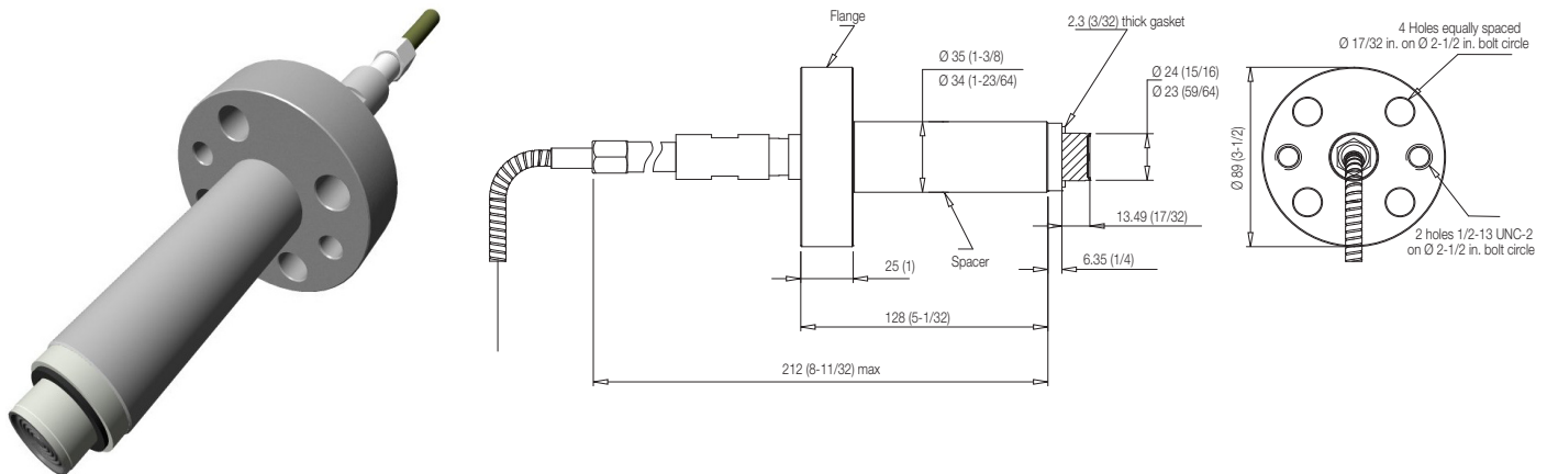
Figure 24: 3-1/4 in. flange extended – type 91 modified
