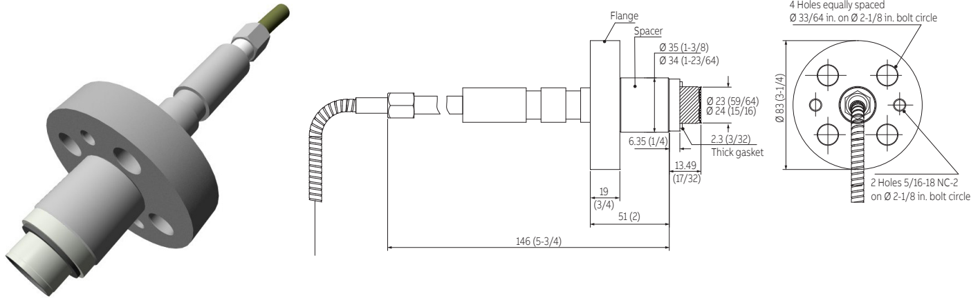
Figure 23: 3-1/4 in. flange extended – type 91
