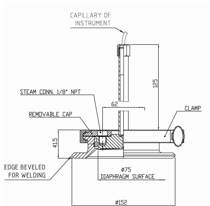
Figure 48: Sanitary spud and welding point
