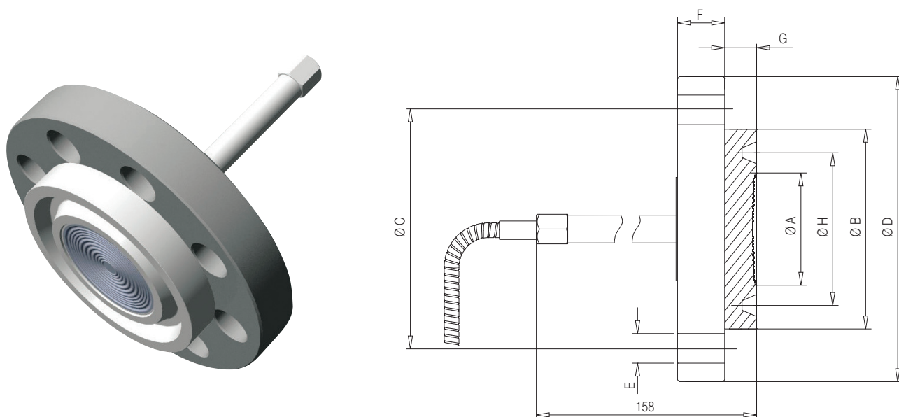
Figure 18: Ring-joint diaphragm seal
