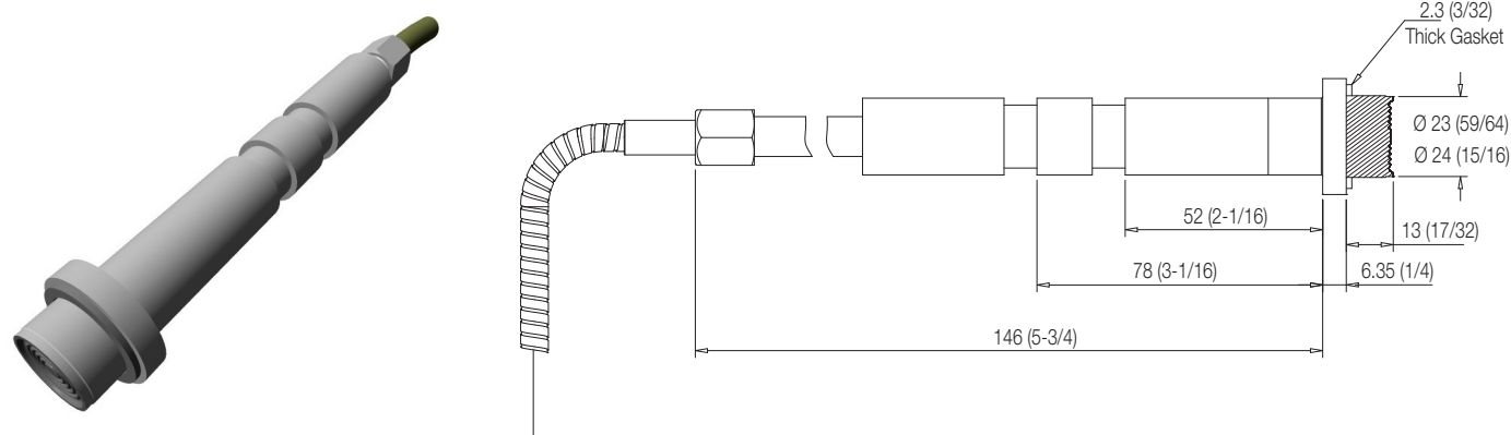
Figure 27: Universal – type 90
