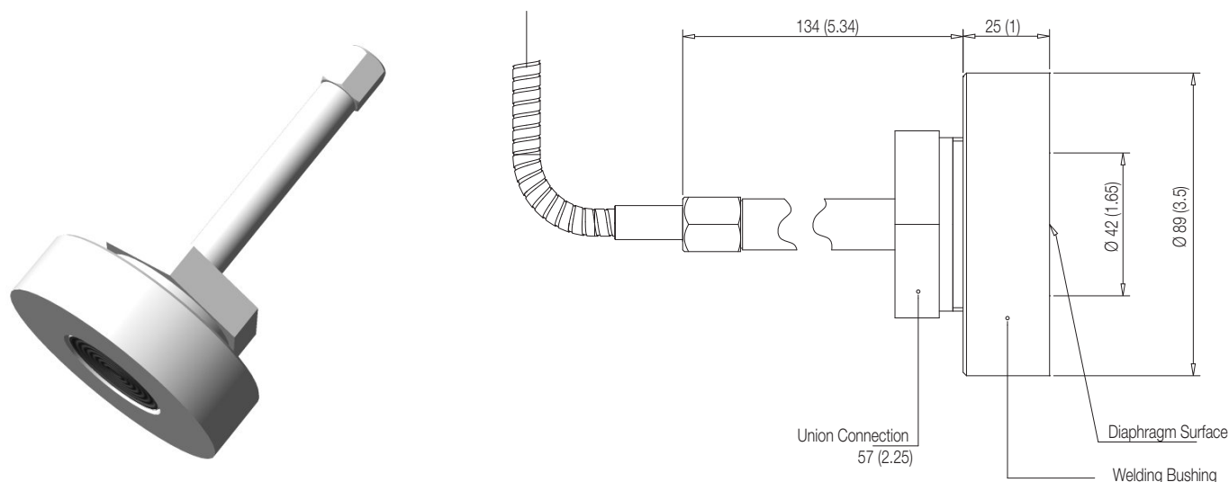
Figure 29: Union connection remote seal with weld bushing
