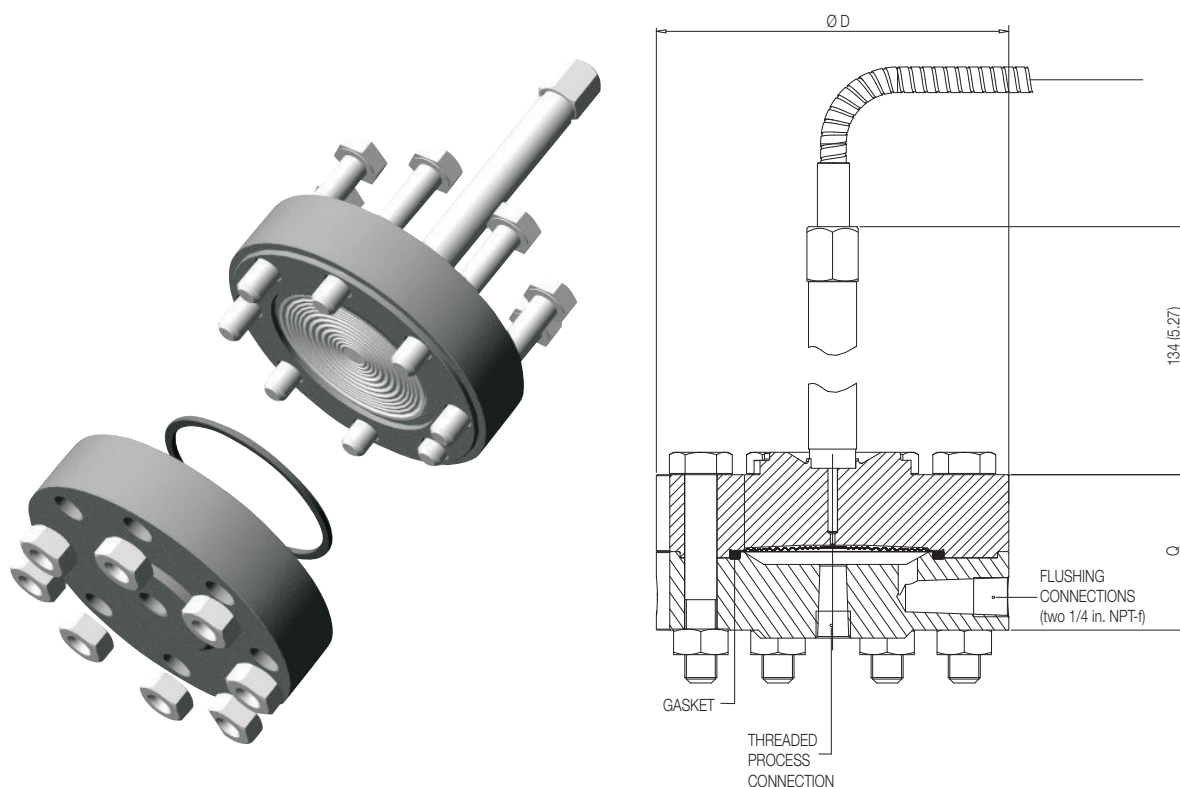
Figure 20: Off-line threaded connection diaphragm seal
